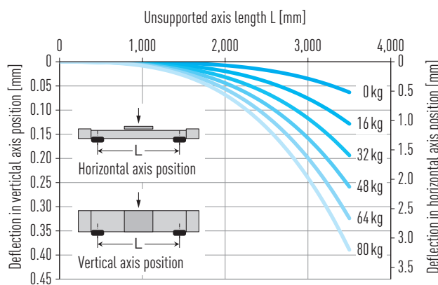
Fig. 8.4 Deflection under load capacity
