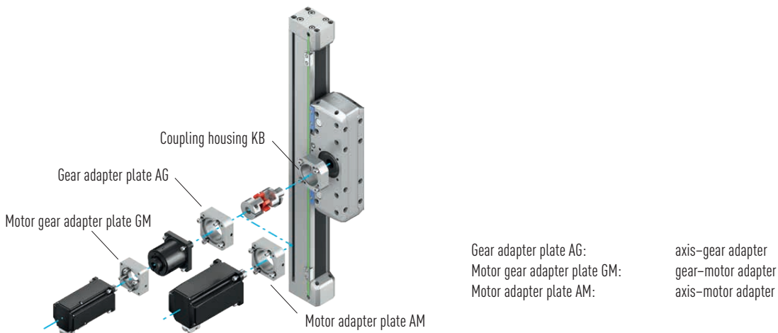
Fig. 16.4 Motor adapter for cantilever axes HC
