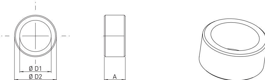
Fig. 17.5 Dimensional drawing of centring sleeve
