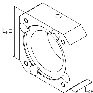
Fig. 16.14 Motor gear adapter plate GM for linear modules HM-B, linear tables HT-B and cantilever axes HC
