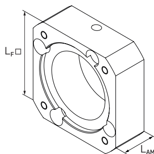
Fig. 16.12 Motor adapter plate AM for linear modules HM-B, linear tables HT-B and cantilever axes HC without gears
