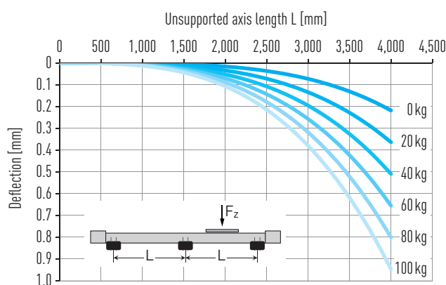
Fig. 6.8 Deflection under load capacity
