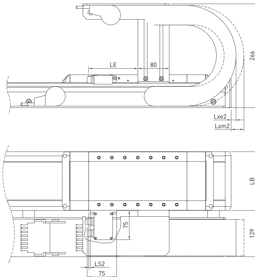
Fig. 16.36 Linear motor axes HT-L: “R” and “B” options – connector right/front, mirrored also applies to “L” and “A” options – connector left/front
