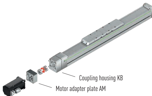
Fig. 16.20 Motor adapter for linear modules HM-S
