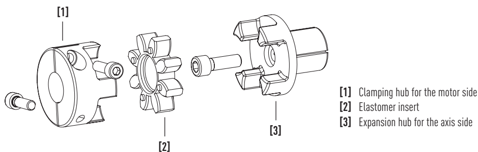
Fig. 16.16 Coupling components for linear modules HM-B, linear tables HT-B and cantilever axes HC
