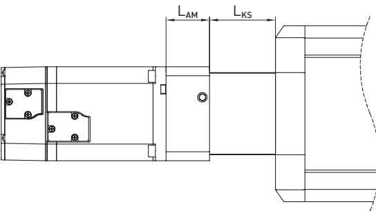
Fig. 16.25 Motor connection of linear tables HT-S without belt drive
