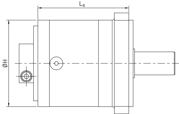
Fig. 16.15 Dimensional drawing of gearbox for linear modules HM-B, linear tables HT-B, cantilever axes HC and double axes HD
