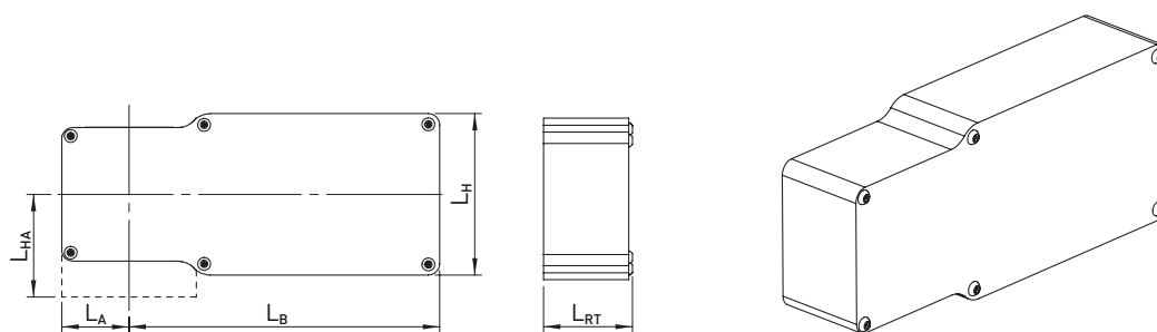
Fig. 16.31 Belt drive RT for linear modules HM-S and linear tables HT-S
