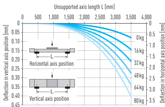
Fig. 9.2 Deflection under load capacity
