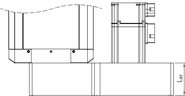
Fig. 16.27 Motor connection of linear tables HT-S with belt drive
