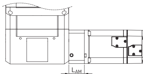
Fig. 16.6 HT-B linear table motor connection without gears
