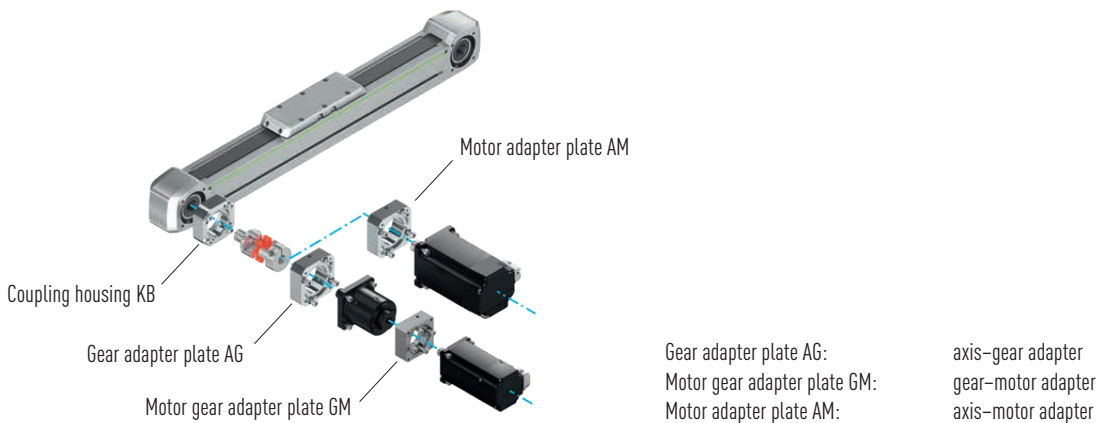
Fig. 16.1 Motor adapter for linear modules HM-B
