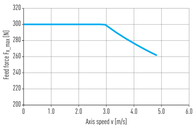
Fig. 5.1 Max feed force F_x as a function of axis speed v
