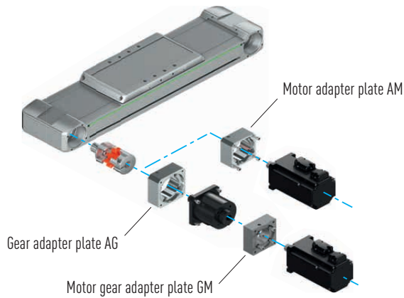
Fig. 16.3 Motor adapter for linear tables HT-B
