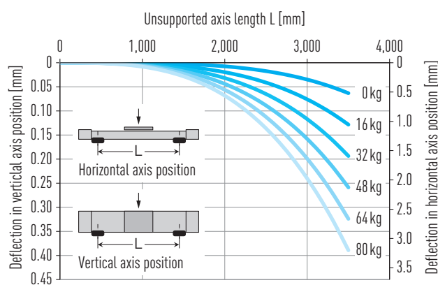
Fig. 7.4 Deflection under load capacity
