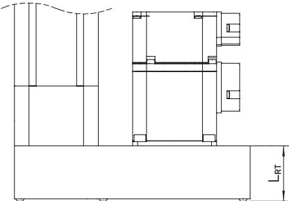
Fig. 16.26 Motor connection of linear modules HM-S with belt drive
