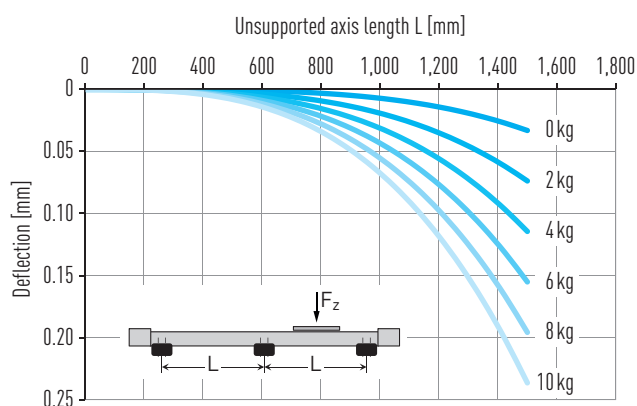
Fig. 5.2 Deflection under load capacity
