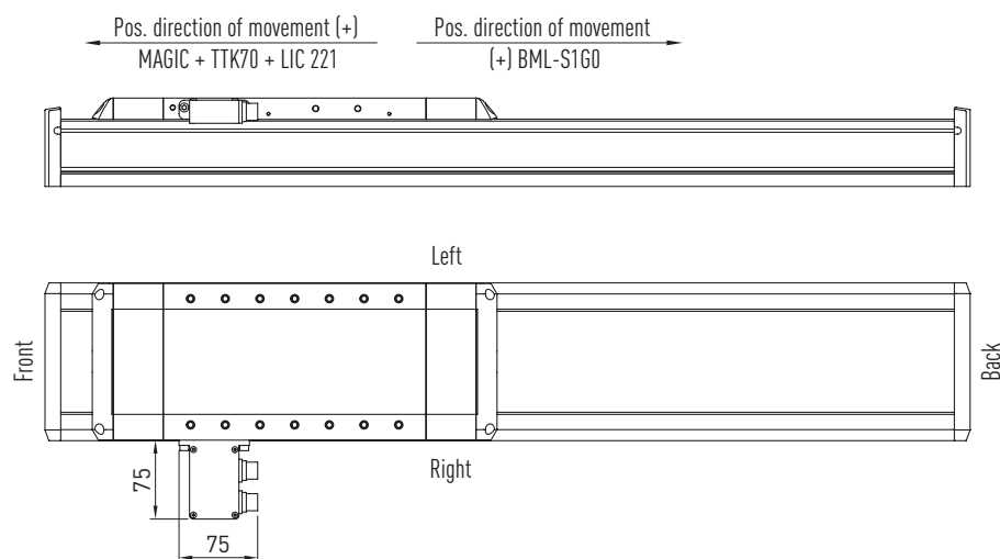
Fig. 15.4 Linear axis HT-L: connection interface "D" – connector right/rear
