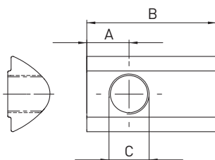
Fig. 17.4 Dimensional drawing of T nut
