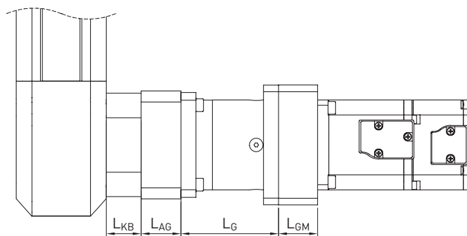
Fig. 16.8 HM-B linear module motor connection with gears
