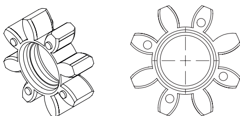
Fig. 16.18 Elastomer insert for linear modules HM-B linear tables HT-B and cantilever axes HC
