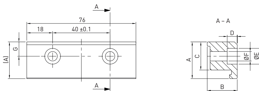
Fig. 17.2 Dimensional drawing of short clamping profile
