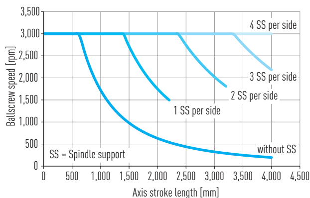
Fig. 8.8 Critical speed
