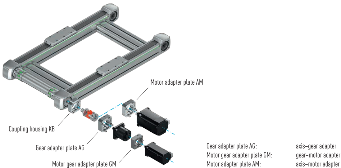
Fig. 16.2 Motor adapter for double axes HD
