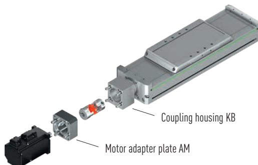
Fig. 16.21 Motor adapter for linear tables HT-S
