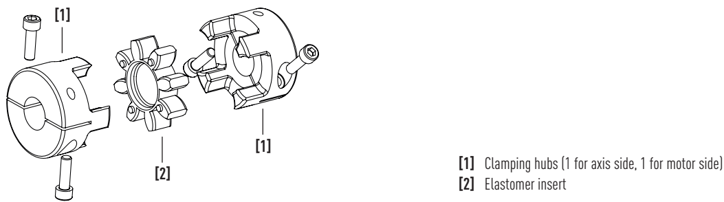
Fig. 16.32 Coupling components for linear modules HM-S and linear tables HT-S
