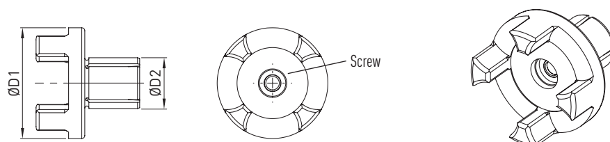
Fig. 16.17 Expansion hub for linear modules HM-B, linear tables HT-B and cantilever axes HC
