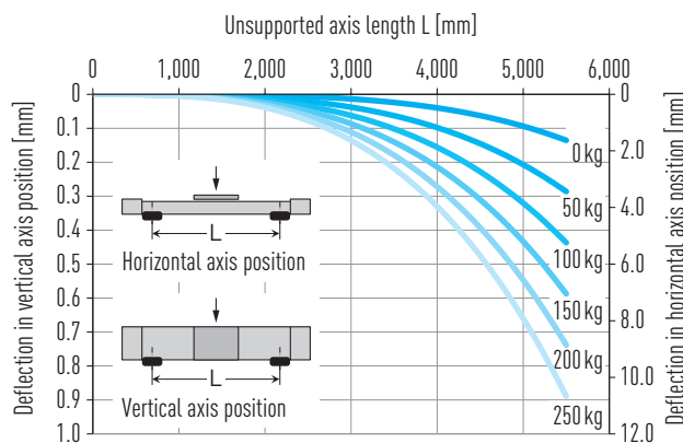
Fig. 8.7 Deflection under load capacity
