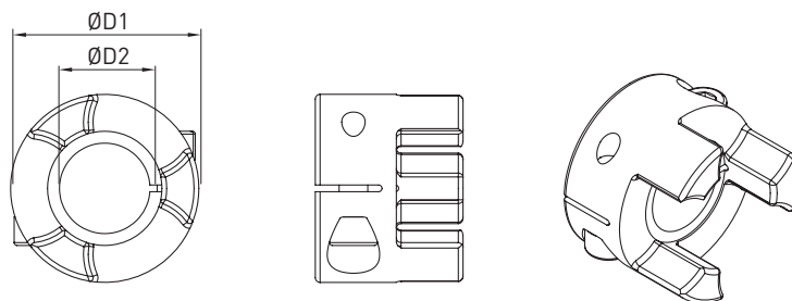
Fig. 16.33 Clamping hub
