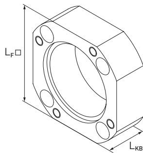
Fig. 16.11 Coupling housing KB for linear modules HM-B and cantilever axes HC
