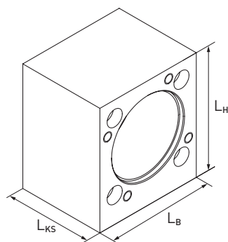
Fig. 16.29 Coupling housing KS for linear tables HT-S
