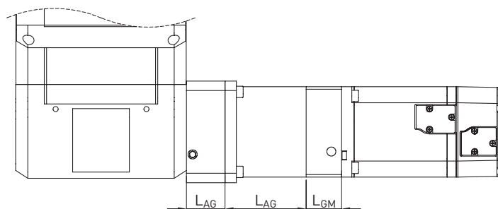
Fig. 16.9 HT-B linear table motor connection with gears
