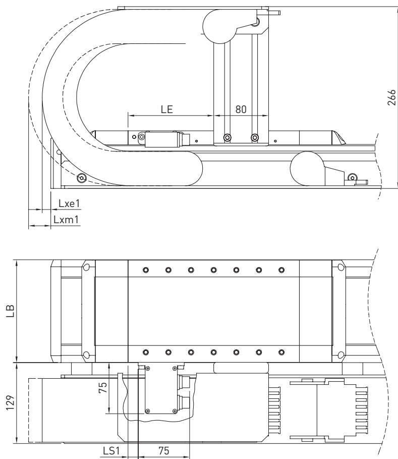
Fig. 16.35 Linear motor axes HT-L: “D” and “F” options – connector right/front, mirrored also applies to “C” and “E” options – connector left/front
