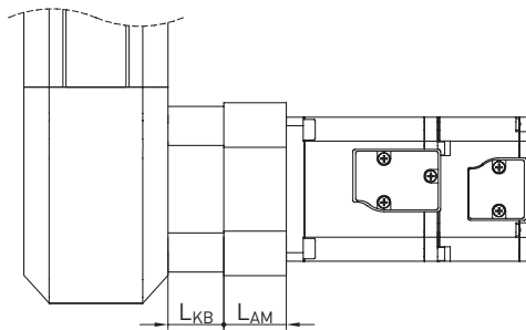
Fig. 16.5 HM-B linear module motor connection without gears
