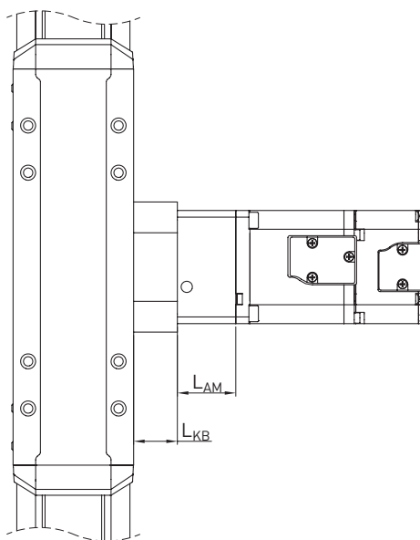
Fig. 16.7 HC cantilever axis motor connection without gears
