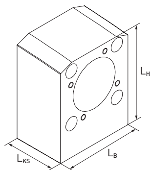
Fig. 16.28 Coupling housing KS for linear modules HM-S
