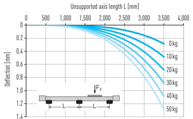
Fig. 5.6 Deflection under load capacity
