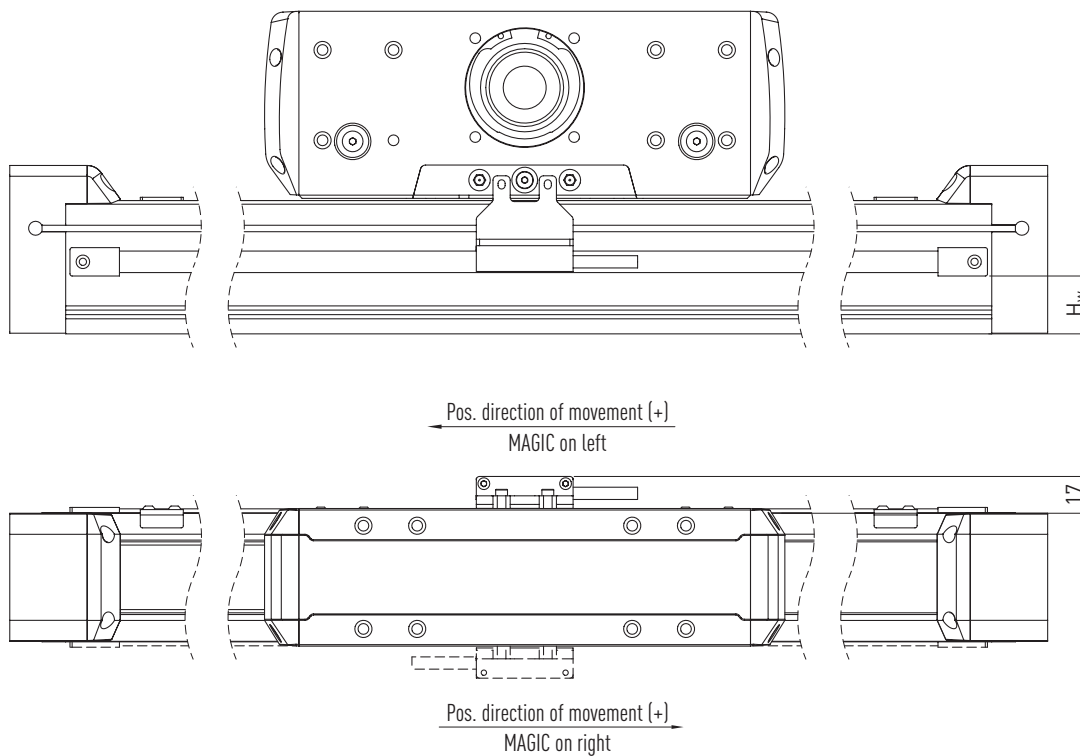
Fig. 15.3 Distance measuring system MAGIC – cantilever axis HC
